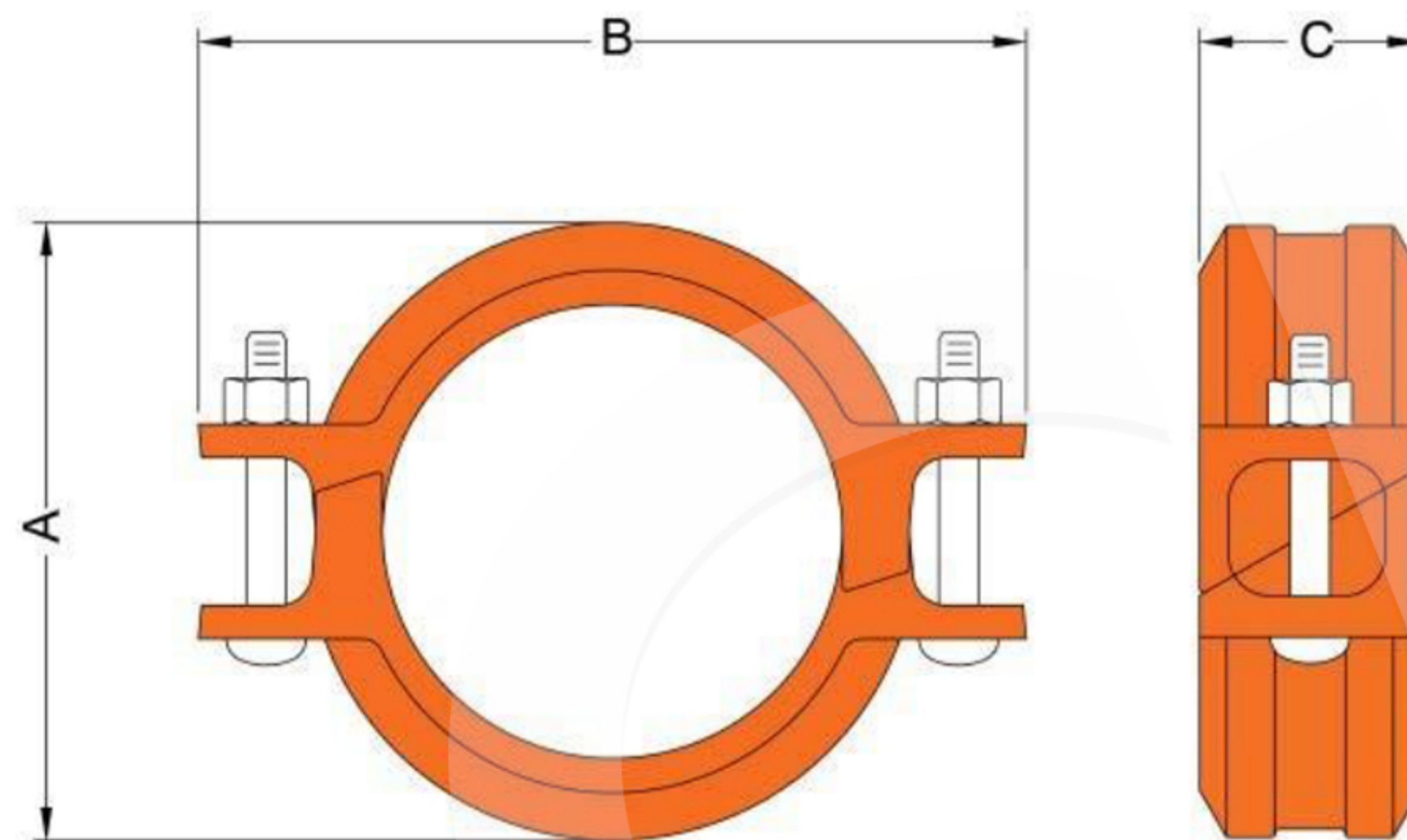
Model Z07 Heavy Duty Rigid Coupling
